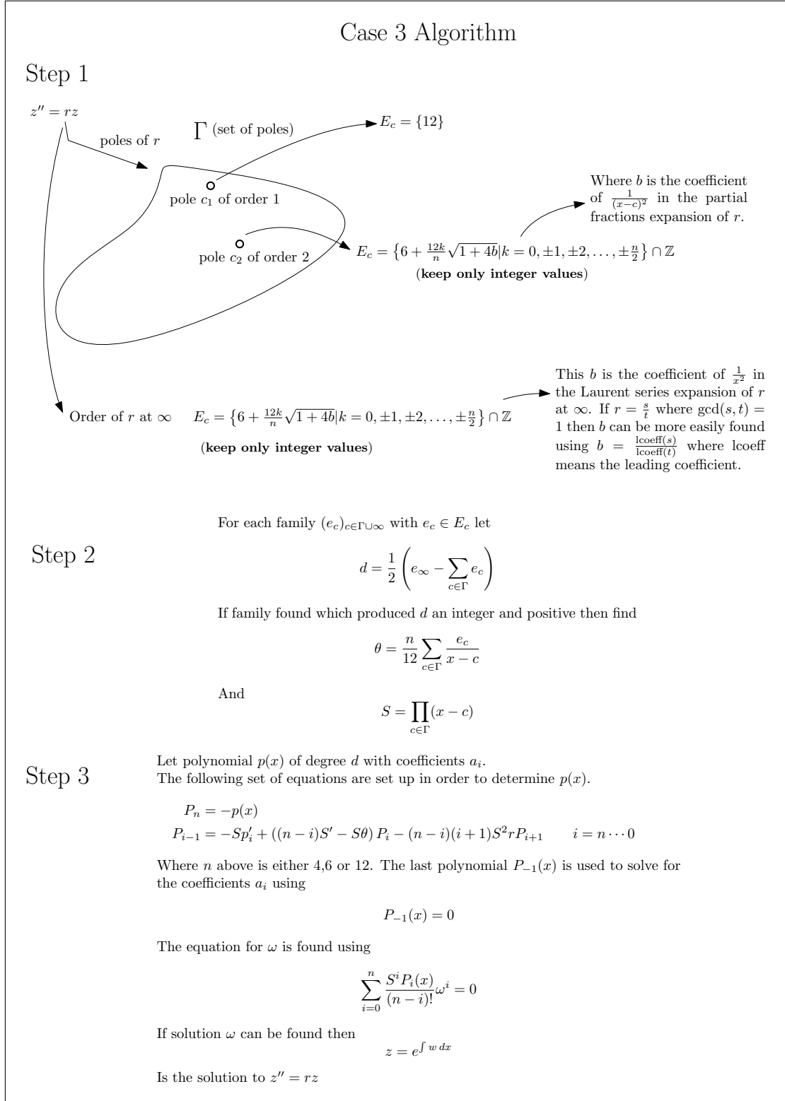
Figure 3: Case 3 Kovacic algorithm
