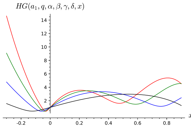
Figure 2: Plot of the general Heun function similar to the one given in [14].
