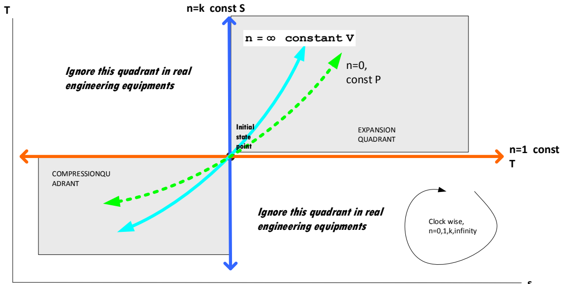
Figure 2: polytropic process diagrams
