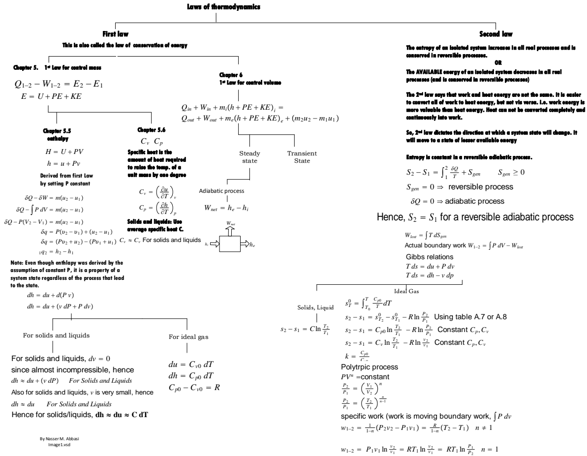
Figure 3: first and second laws diagrams
