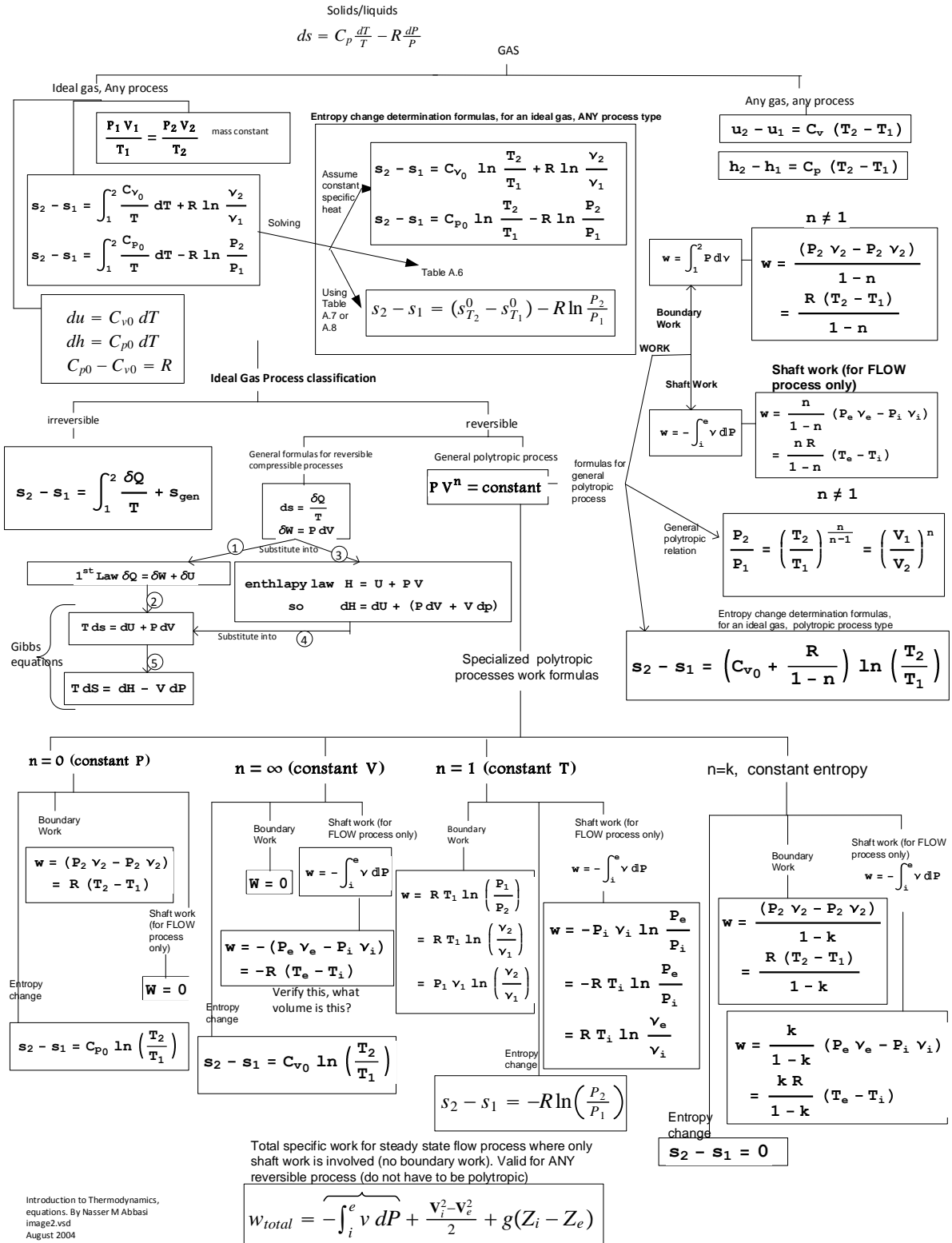
Figure 4: gas laws
