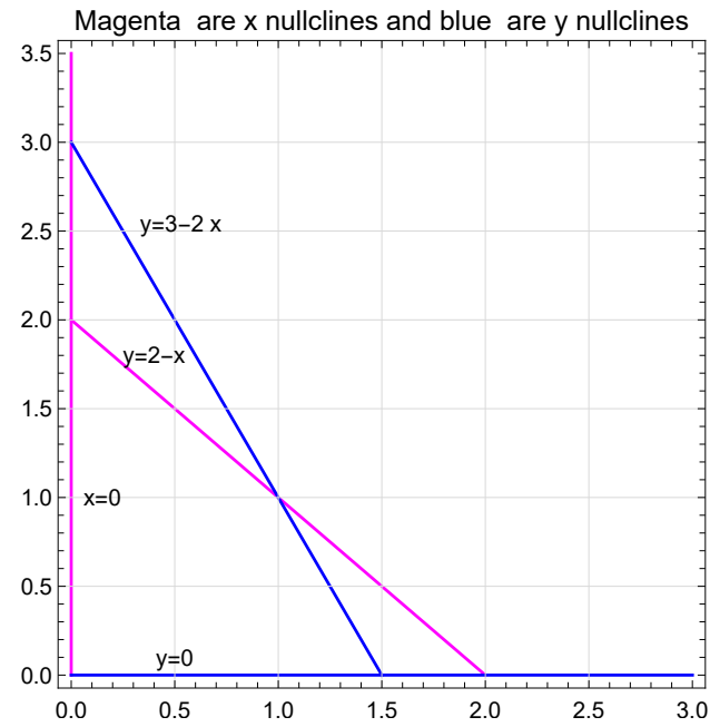
Figure 1: nullclines lines
