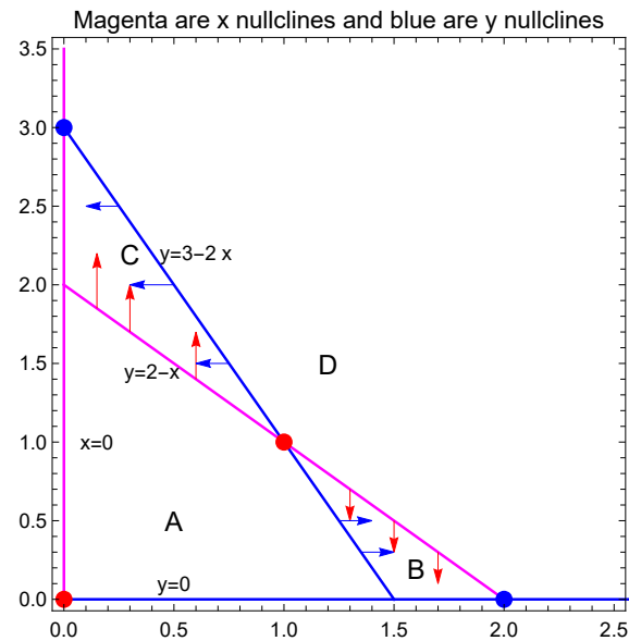
Figure 5: Direction fields based on y nullcline analysis
