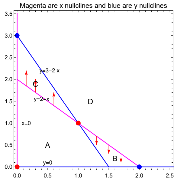
Figure 4: Direction fields based on x nullcline analysis
