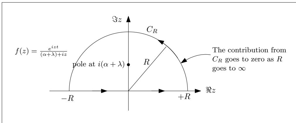
Figure 3: Contour integration used for finding inverse Fourier transform
