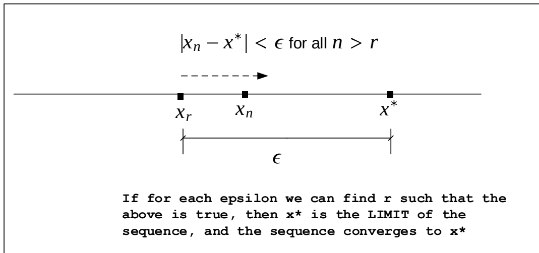
Figure 3.8: example
