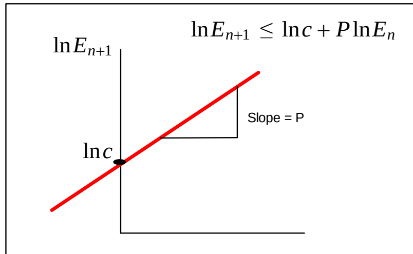
Figure 2.6: Plot
