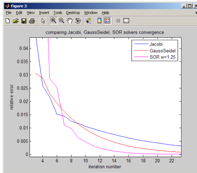
Figure 4.6: SOR plot
