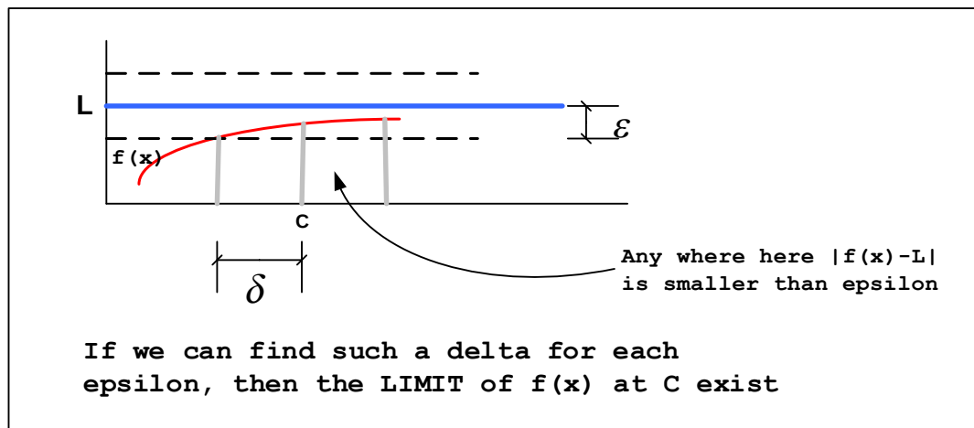
Figure 3.1: Limit
