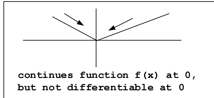
Figure 3.5: example
