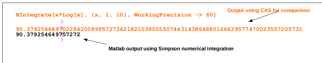
Figure 4.8: Result
