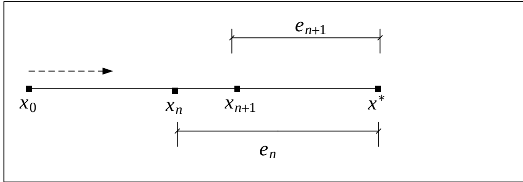
Figure 3.9: example
