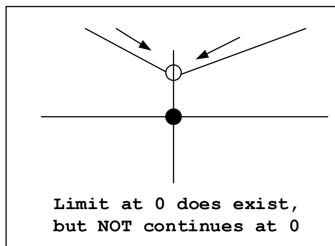
Figure 3.3: example
