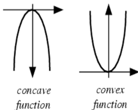
Figure 3.13: Mathworld
