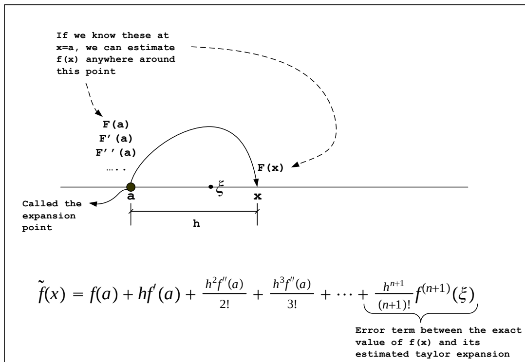
Figure 3.7: example
