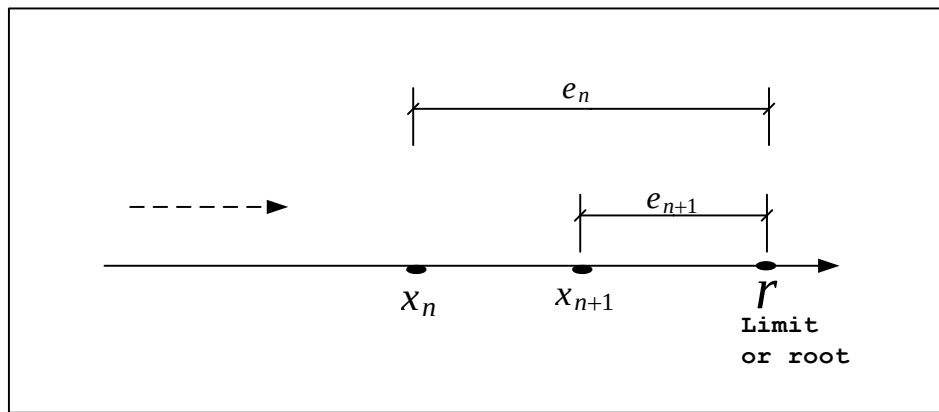
Figure 3.12: quadratic convergence
