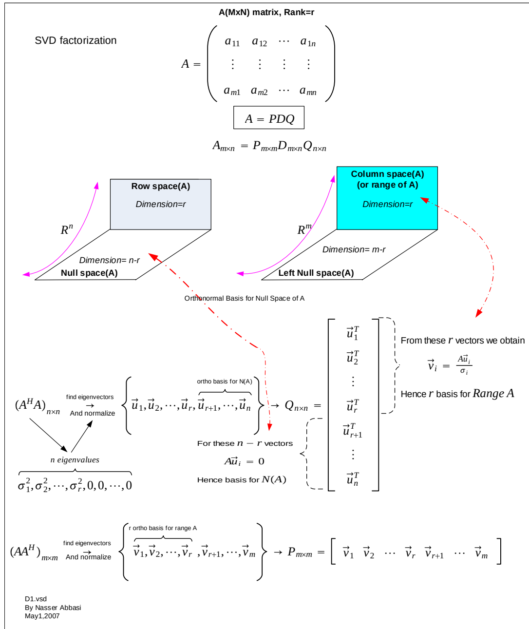
Figure 2.1: SVD
