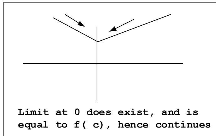
Figure 3.4: example
