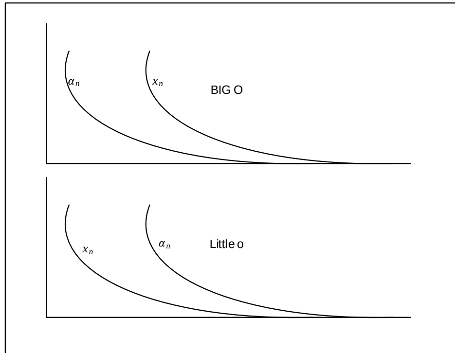
Figure 3.11: example
