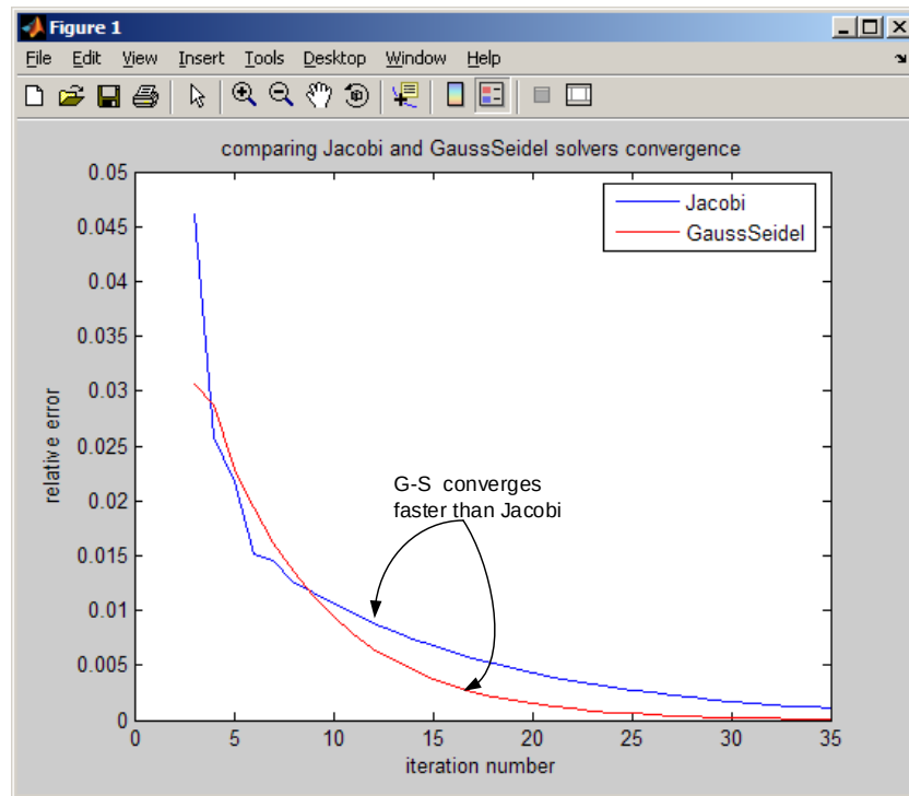
Figure 4.3: Plot
