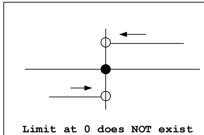
Figure 3.2: example
