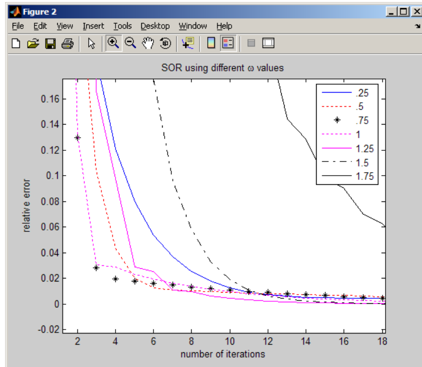
Figure 4.5: Zoom plot
