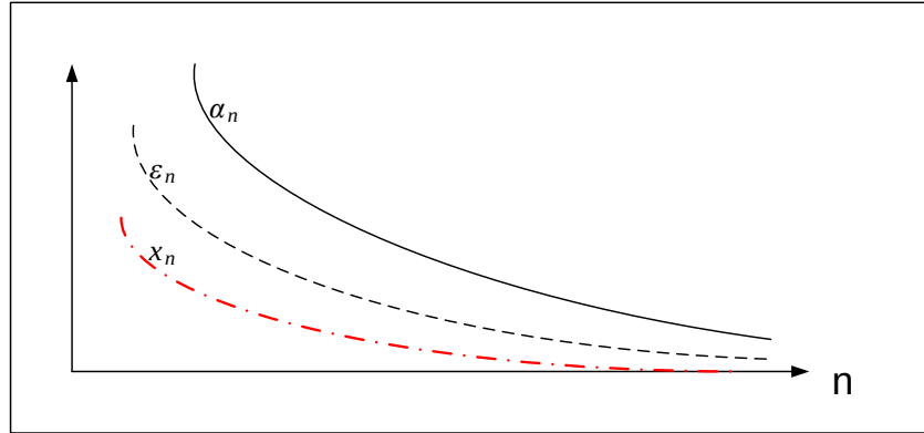
Figure 2.7: Plot
