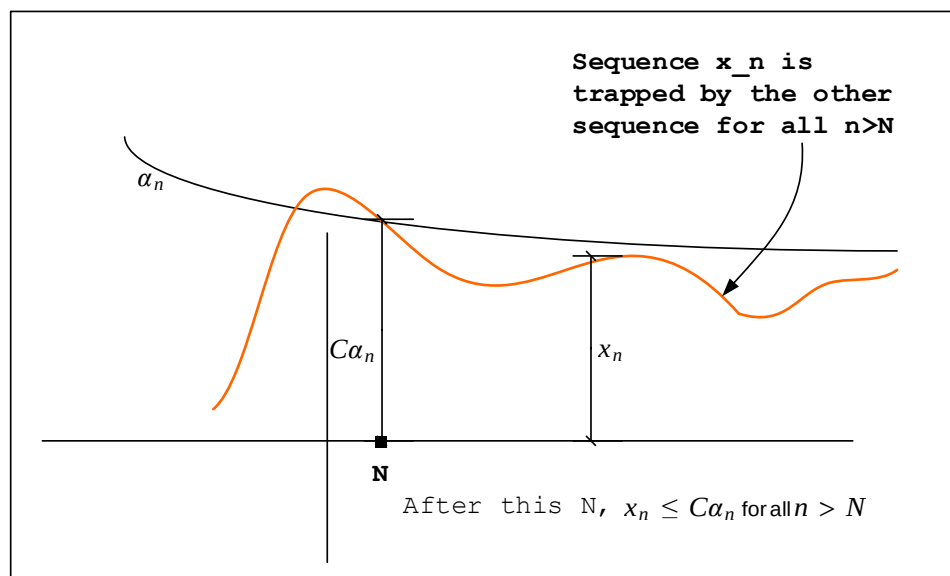
Figure 3.10: example
