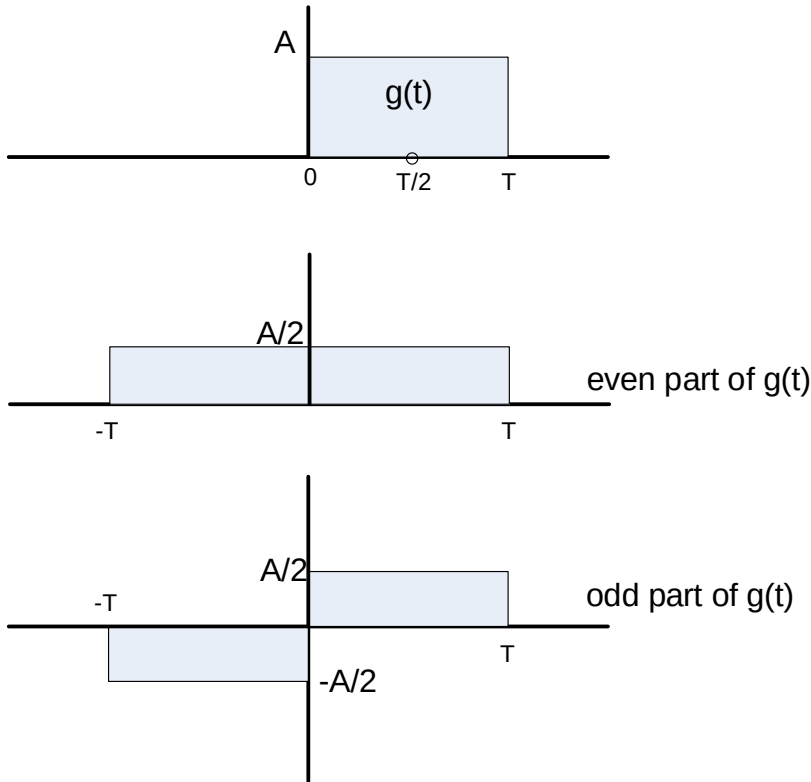
Figure 3.1: rectangular pulse
