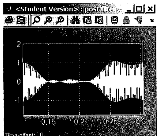
Output of digital filter inside the demodulator
